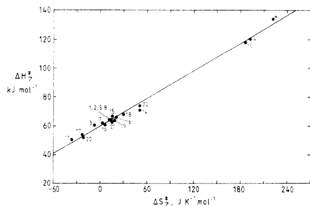
Figure 4. Plot of \Delta H_7^\ddagger vs. \Delta S_7^\ddagger for various CO 2 uptake reactions. (See Table XXXI for the data numbering system.)
