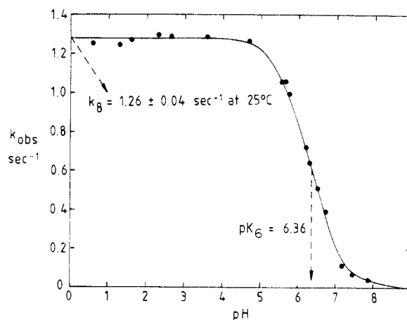
Figure 5. Plot of k_{obsd} vs. pH for the reaction trans\text{-Rh(en)}_2(\text{Cl})\text{OCO}_2 + \text{H}^+ \rightarrow trans\text{-Rh(en)}_2(\text{Cl})\text{OH}^+ + \text{CO}_2 at 25 °C and an ionic strength of 0.5 M. Data taken from ref 315.
